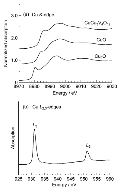
Figure 2. a) Room-temperature XAS spectra at the Cu K-edge for \text{CuCu}_3\text{V}_4\text{O}_{12} and standards ( \text{CuO} and \text{Cu}_2\text{O} ); spectra vertically offset for clarity. b) Room-temperature XAS spectrum at the Cu L_{2,3} -edges for \text{CuCu}_3\text{V}_4\text{O}_{12} .
